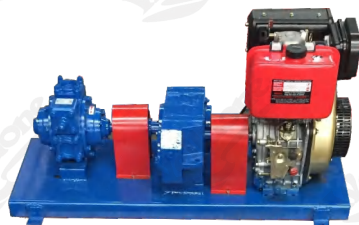
带联轴器连接 with coupling connect
